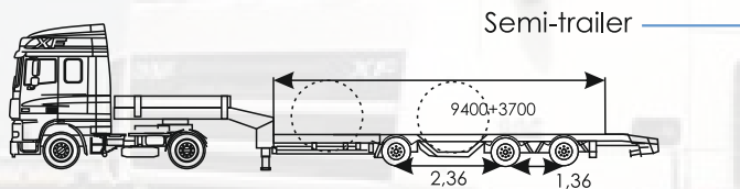
Multiplus-3 up to 23 t
