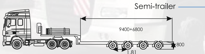
Multimax-4 - up to 30 t
