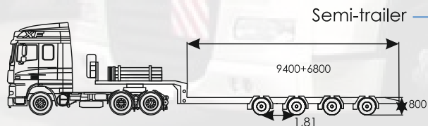
Multimax-4 - up to 30 t
