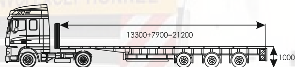
Telemax-3 up to 20 t
