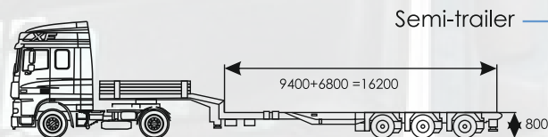
Multimax-3 up to 23 t
