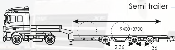
Multiplus-3 up to 23 t
