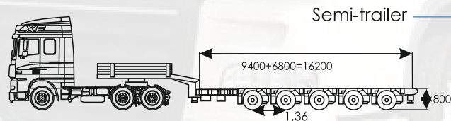
Multimax-5 up to 38 t
